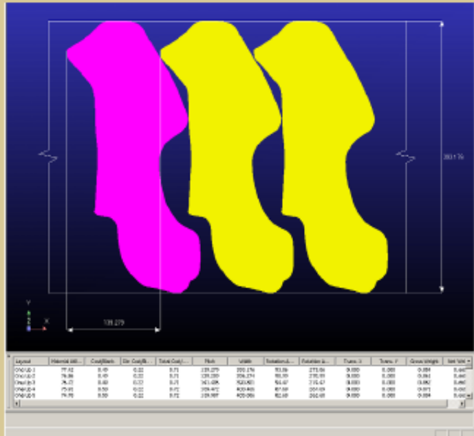
1 Up Blank Nesting Layout
